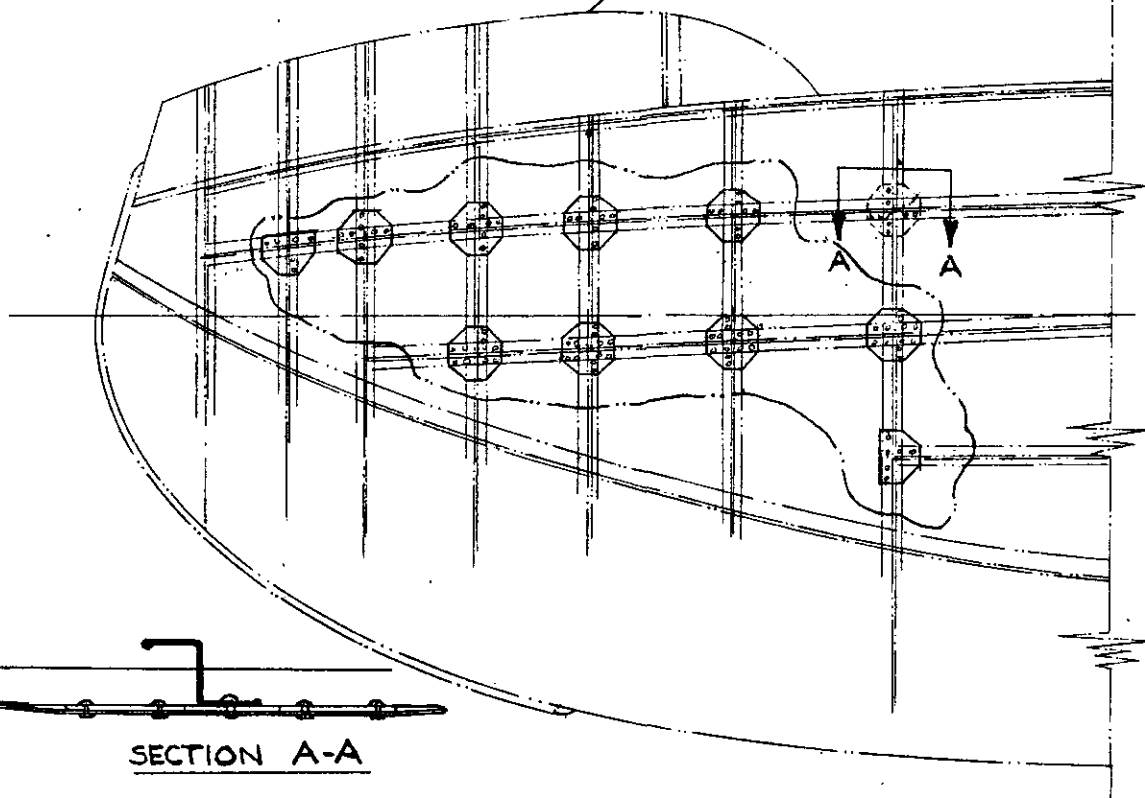
FIG. 35 - TYPICAL METHODS OF REPAIRING CRACKED FRAME AND STIFFENER COMBINATIONS.
