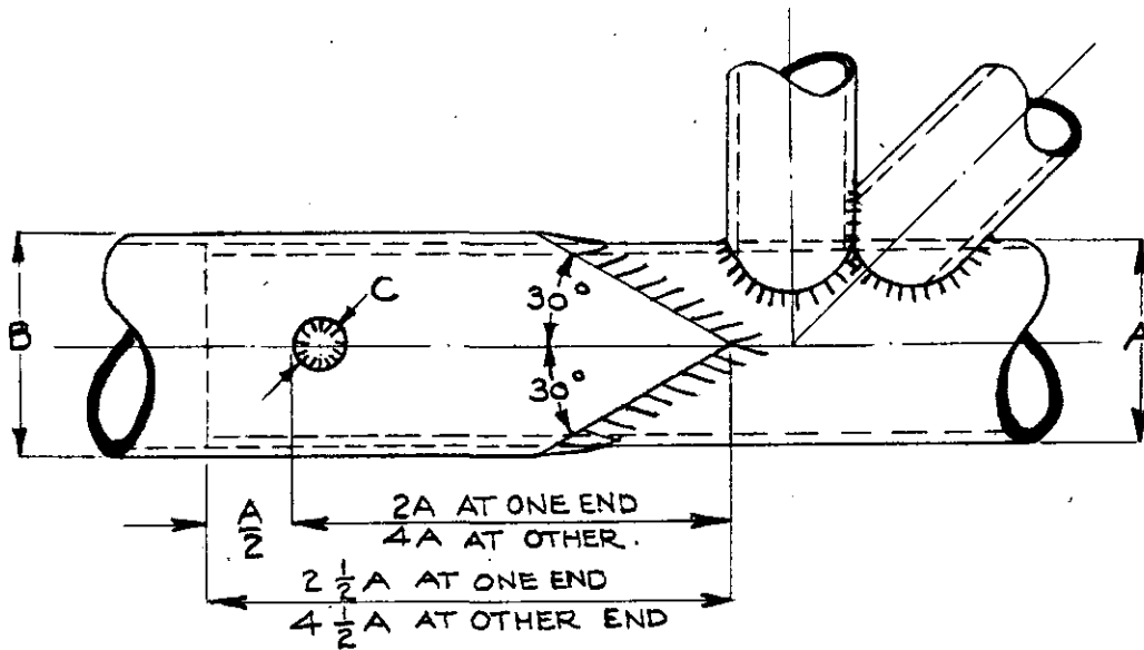
FIG. 21 - ENGINE MOUNT AND LONGERON REPAIR USING LARGER DIAMETER REPLACEMENT TUBE.
