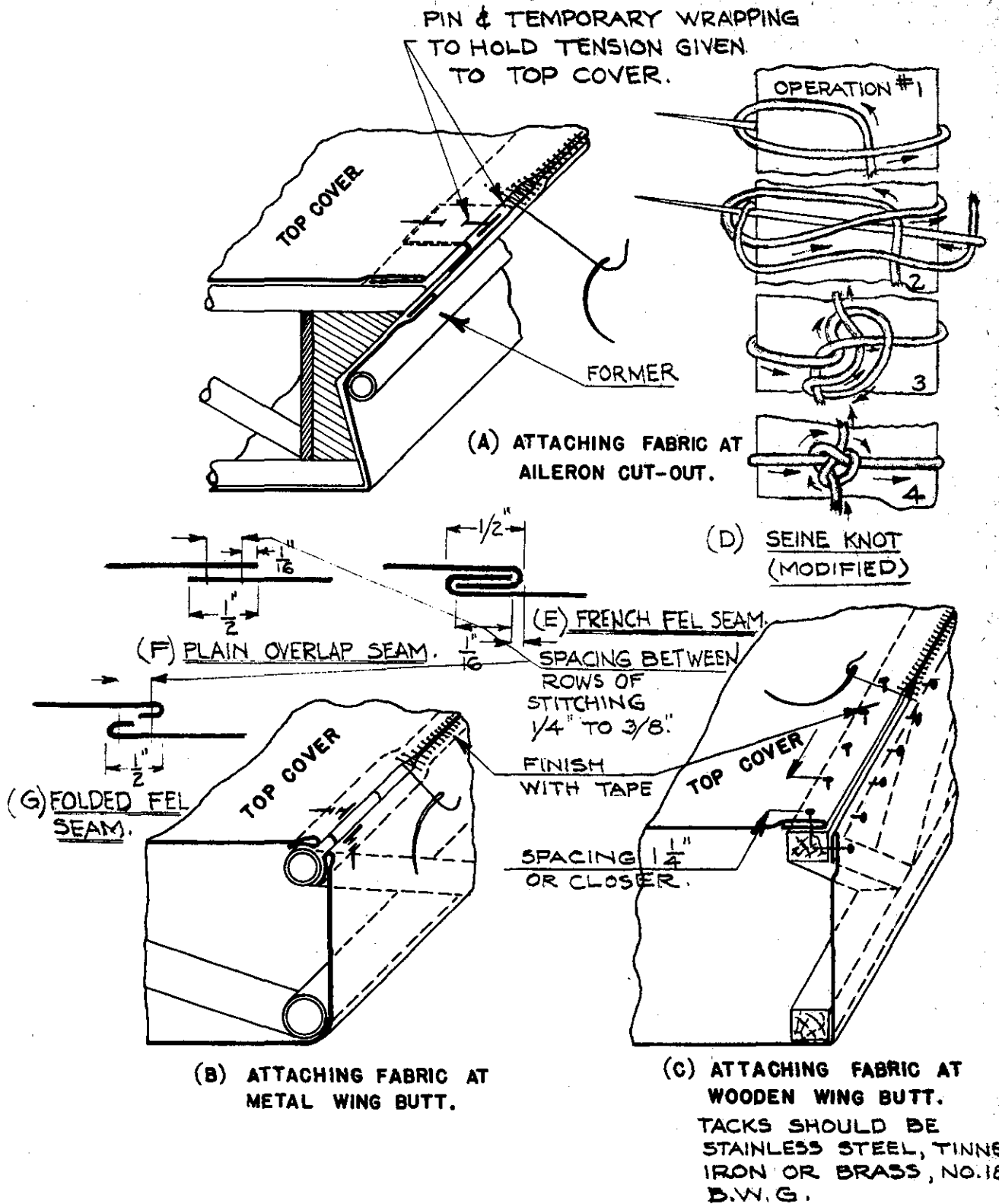
FIG. 16 - TYPICAL METHODS OF ATTACHING FABRIC .
