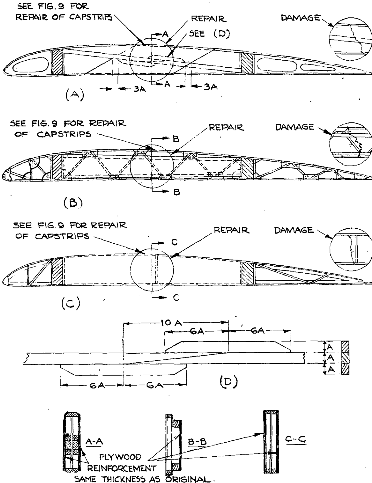
FIG. 11 - TYPICAL WING COMPRESSION RIB REPAIRS Reference - Section 18.6017
