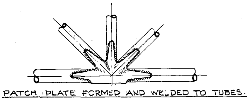
FIG. 17 - REPAIR OF A LONGERON DAMAGED AT A STATION USING A PATCH PLATE. Reference - Section 18.6110
