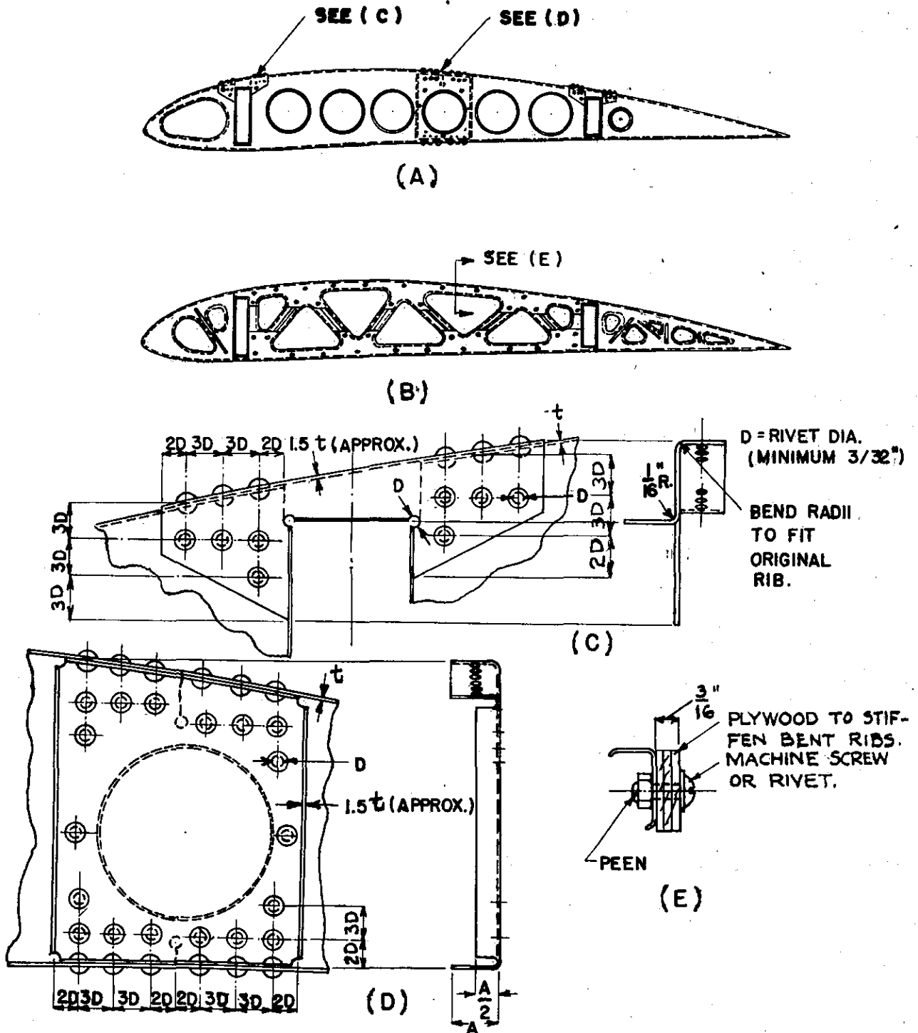
FIG. 30 - TYPICAL METAL RIB REPAIRS (COMMONLY FOUND ON SMALL AND MEDIUM SIZE AIRCRAFT.) Reference - Section 18.6442
