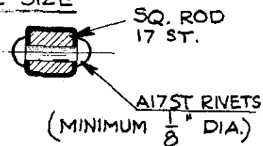
FIG. 29 TYPICAL REPAIR FOR BUCKLED OR CRACKED FORMED METAL WING RIB CAPSTRIPS.*
