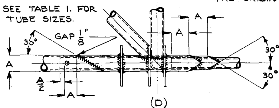
FIG. 22 - ALTERNATE TYPICAL REPAIRS AT A FITTING.
