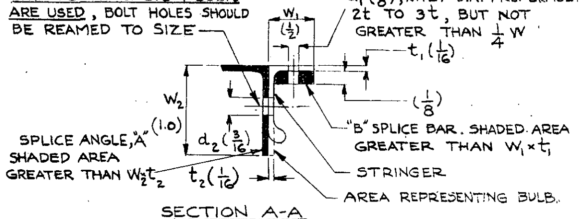
FIG. IV - EXAMPLE OF STRINGER SPLICE (MATERIAL - 17ST AL. ALLOY)
