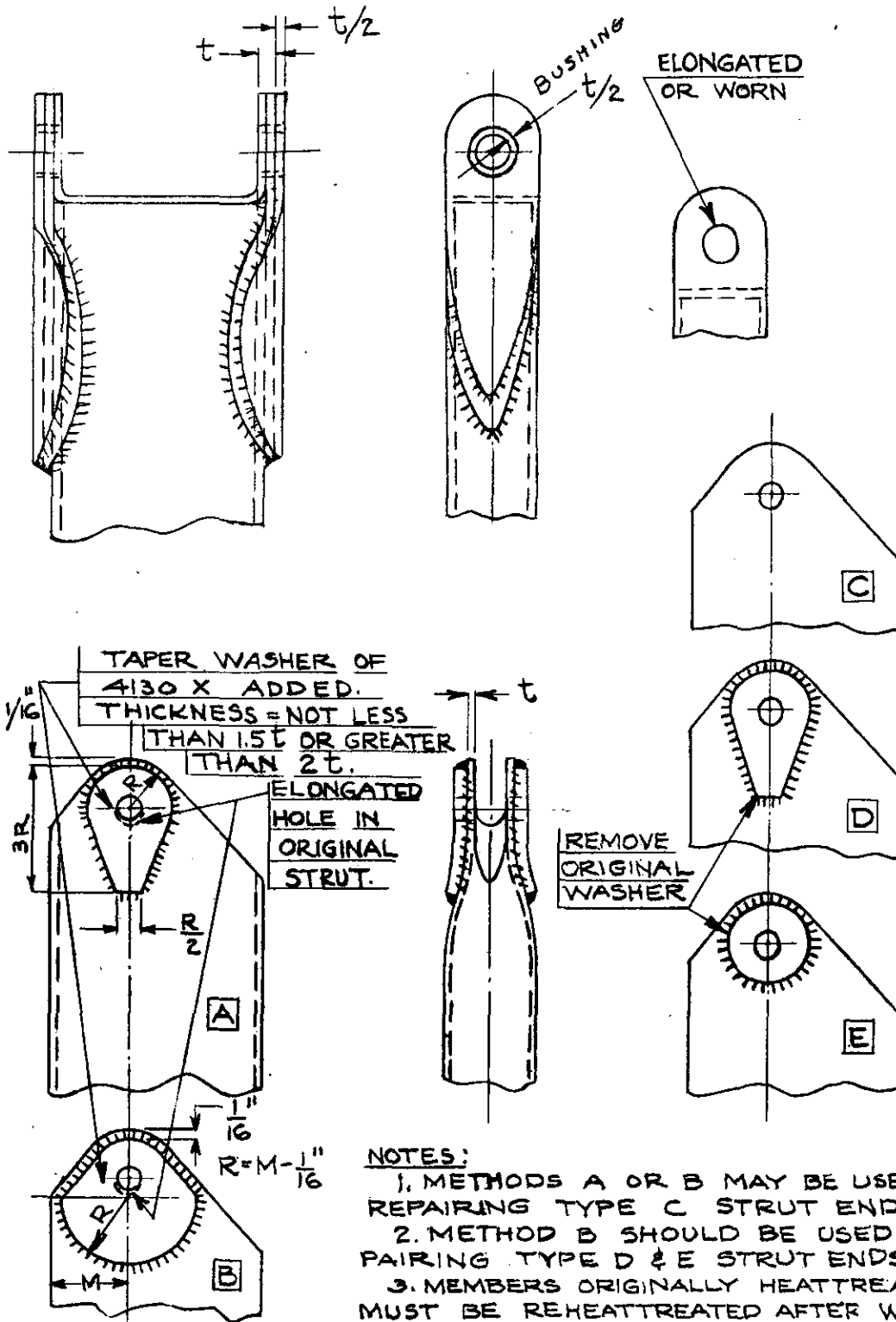
FIG.13 - TYPICAL METHODS OF REPAIRING ELONGATED OR WORN BOLT HOLES Reference - Section 18.6042
